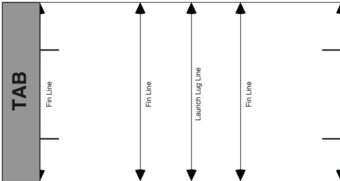
T-60 Three Fin Tube Marking Guide
