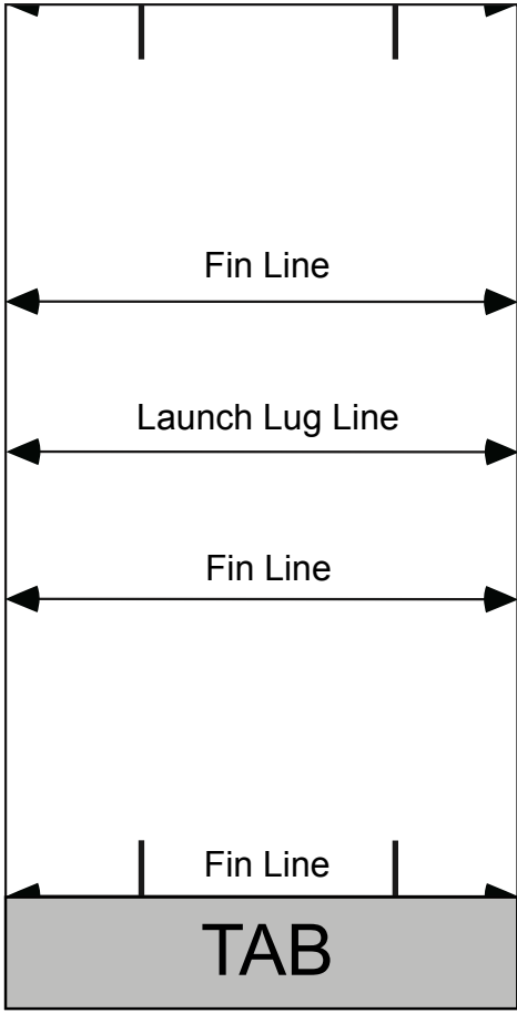
T-55 Three Fin Tube Marking Guide
