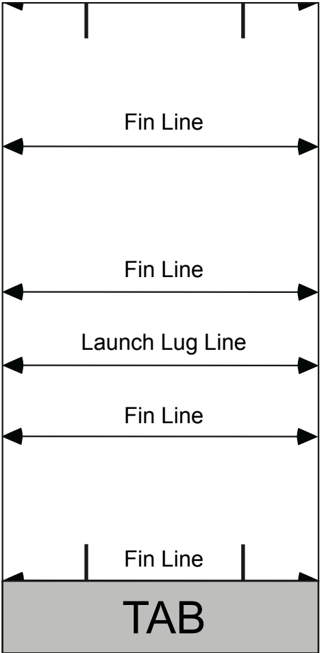
TT-55 Four Fin Tube Marking Guide
