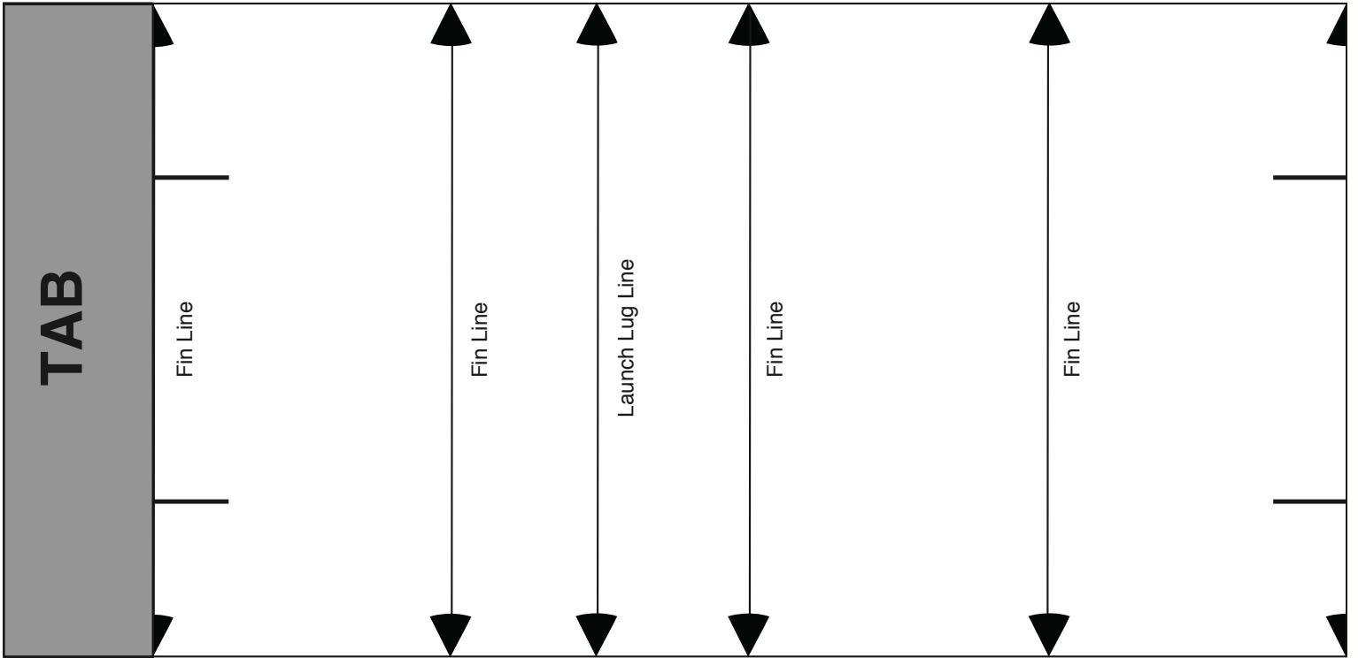
T-70 Four Fin Tube Marking Guide
