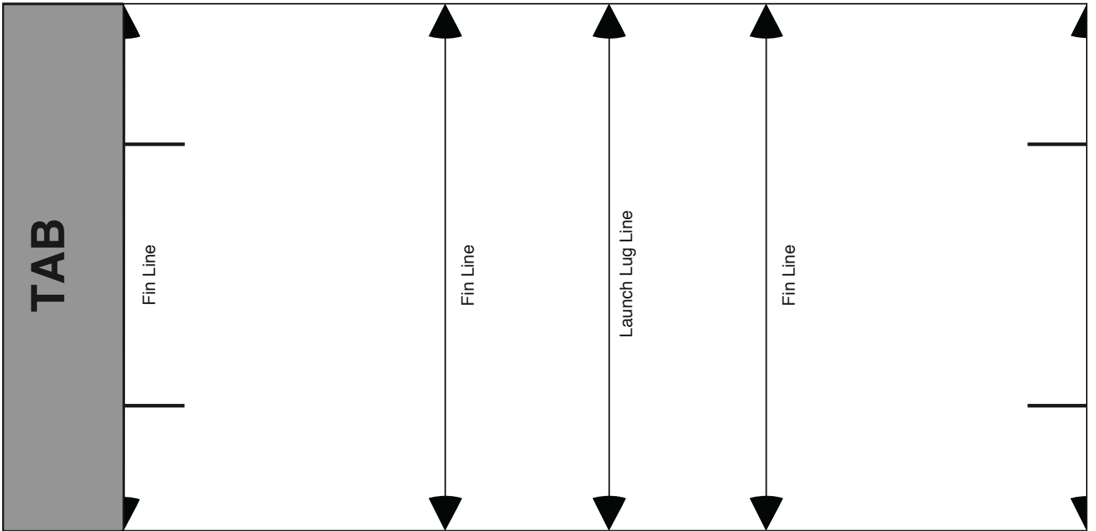
T-70 Three Fin Tube Marking Guide
