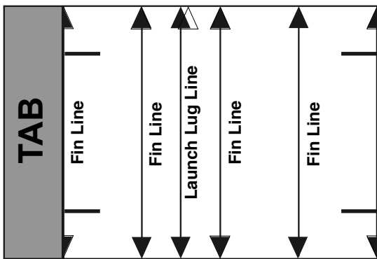
Two High! 4 Fin Tube Marking Guide
